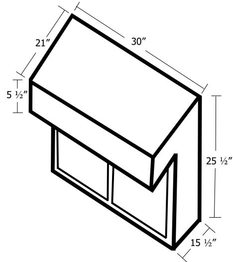
30" Barrier Free Vanity cabinet diagram shown from top side view with dimensions
